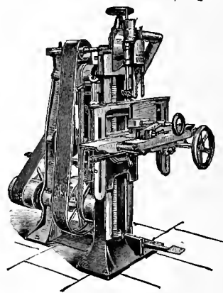
Standard Chain Saw Mortiser.
